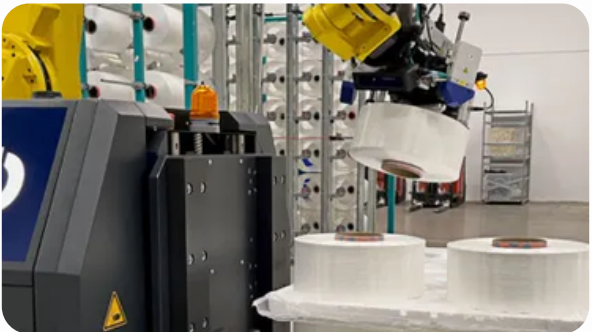
Robotic assistance system Using 3D camera to send position data for the automated placement of products
