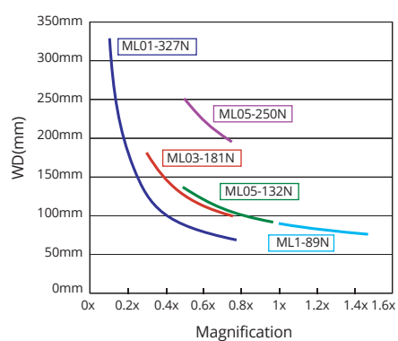
Reference magnification and WD data for close-up ring combinations
